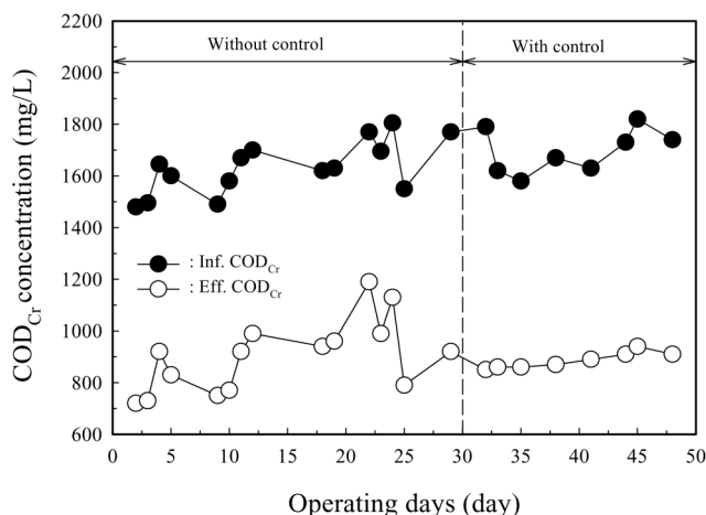
Fig. 7. Influent and effluent COD Cr concentration in the oxidation reactor of the pilot scale Fenton oxidation process with and without the control system using ORP measurements ( \text{Fe}^{2+}/\text{H}_2\text{O}_2 molar ratio, 0.3; pH, 3).
